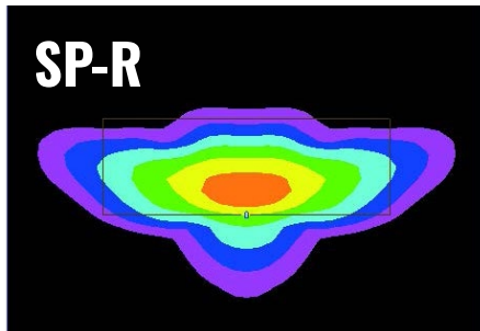
SP-R Optics for very narrow roads with normal pole spacing. Highly energy efficient.
