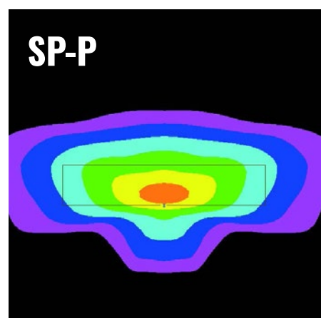
Even general optics for lighting both sides of the road or ramps. Suitable for very long pole spacing. Best installed away from the road.
