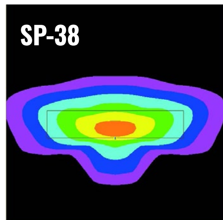
Highway optics to be installed on the middle area. Especially suitable for high poles and extra long, up to 100 meter, pole spacing.
