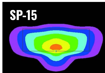
SP-15 General optics for roads with very long pole spacing. Offers even light also in wet conditions. Relatively wide road profile (lits also opposite cycleways if the pole spacing is short)
