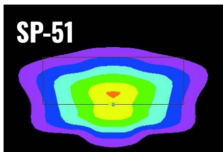
SP-51 A lot of back area light optic for long pole spacing. Energy efficient if cycleways is located behind the poles
